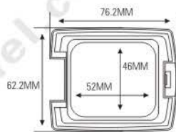
ES1116 SIZE: L76.2×W62.2×H21.4mm
