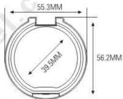
ES1072 SIZE: L55.3 \times W56.2 \times H24.5 mm
