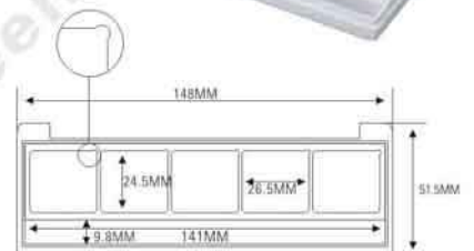
ES1011-5FTSNB(ES1011C-5FY) SIZE: L148×W51.5×H12.5mm
