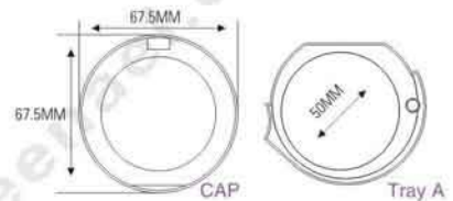
ES1102 SIZE: \varnothing 67.5 \times H37\text{mm}
