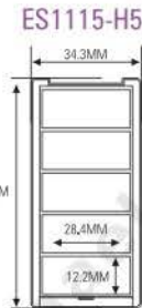
ES1115 ES1115-H5 ES1115-H4 SIZE: L34.3×W75×H17.7mm 75MM
