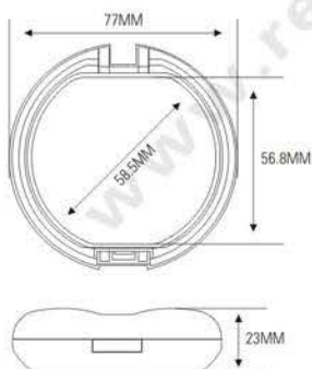
ES1019 SIZE: \varnothing 77 \times H23 mm
