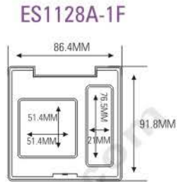
ES1128A-1F ES1128A-2F ES1128A-4F SIZE: L86.4×W91.8×H15.4mm
