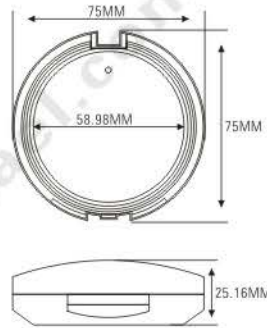
ES1106B SIZE: \varnothing 75 \times H 25.16\text{mm}
