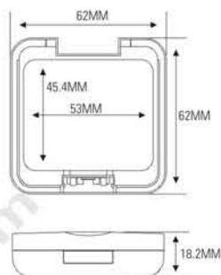
ES1020 SIZE: L62 \times W62 \times H18.2 mm
