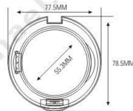
ES1075 SIZE: L77.5 \times W78.5 \times H21.5 mm
