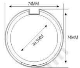
ES1125 (ES1125P) SIZE: \varnothing 74 \times H28.75\text{mm}
