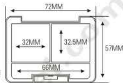
ES1051-2 ES1051-4 SIZE: L72×W57×H15.5mm
