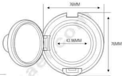
ES1098 SIZE: \varnothing 76 \times H26.1\text{mm}
