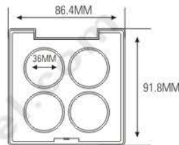
ES1128B-4Y SIZE: L86.4×W91.8×H15.4mm
