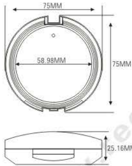
ES1106 SIZE: \varnothing 75 \times H 25.16\text{mm}
