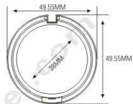
ES1036A SIZE: \varnothing 49.55 \times H18.31\text{mm}
