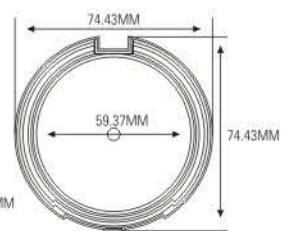
ES1105 SIZE: Ø74.43 x H20.8mm
