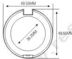
ES1036B SIZE: \varnothing 49.55 \times H21\text{mm}
