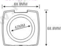
ES1127-1Y42
