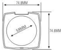
ES1152-1Y59 ES1152W-1Y59
