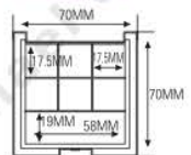
ES1086-6FS(ES1086A1-7) ES1086L-6FS
