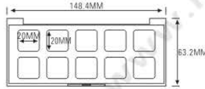
ES1167-10F20
